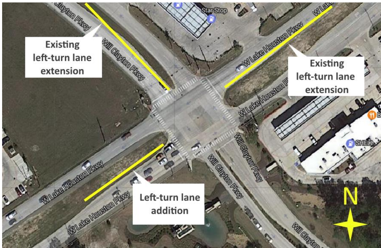
Planned intersection modifications for West Lake Houston Parkway at Will Clayton Parkway.
